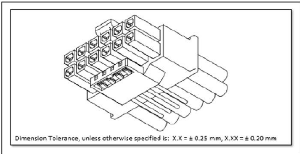
Figure 5-3: 12VHPWR Cable Plug Connector
